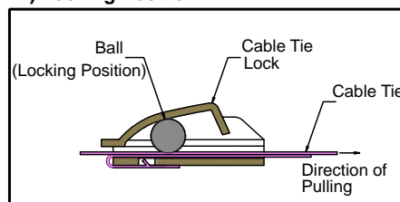
2) Locking Position
